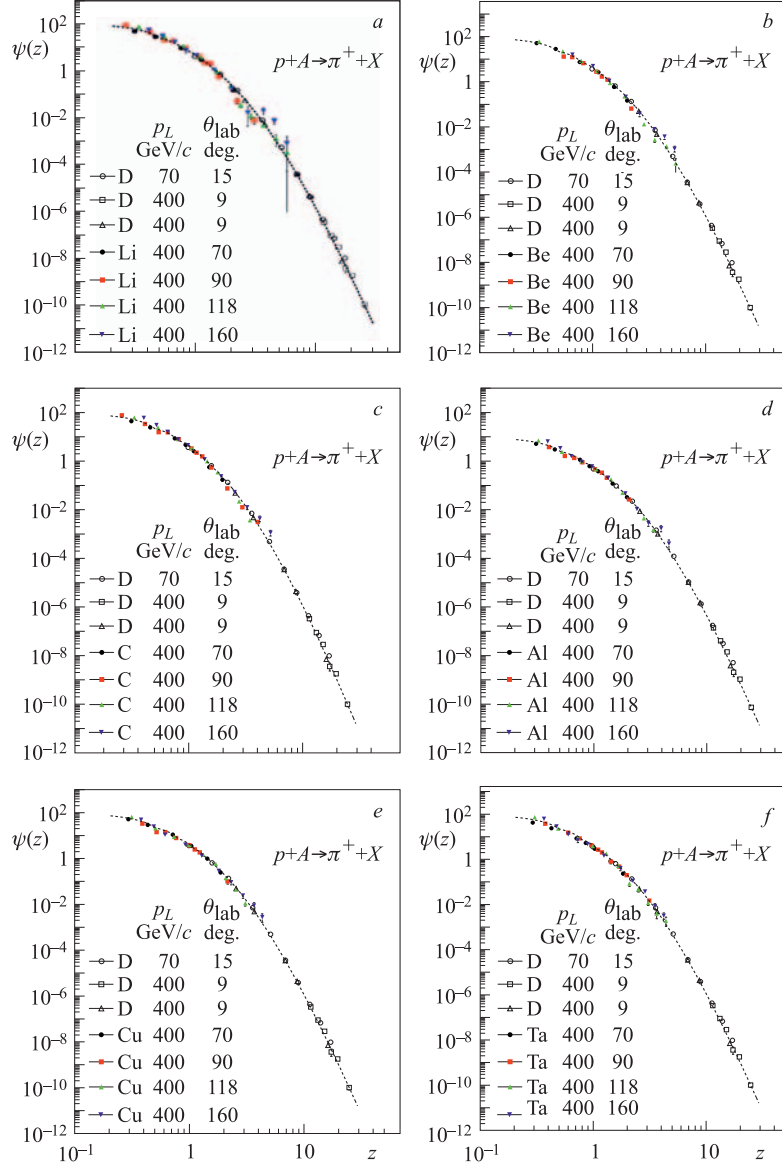
Fig. 3. Scaling function \psi(z) versus variable z for the \pi^+ mesons produced in p + A collisions at momentum p_L = 400 GeV/c and angle \theta_{\text{lab}} = 70, 90, 118 and 160^\circ . The dotted line is the result of fitting. It is the same on all graphs. The points are z presentation of the experimental data taken from [27–30]
