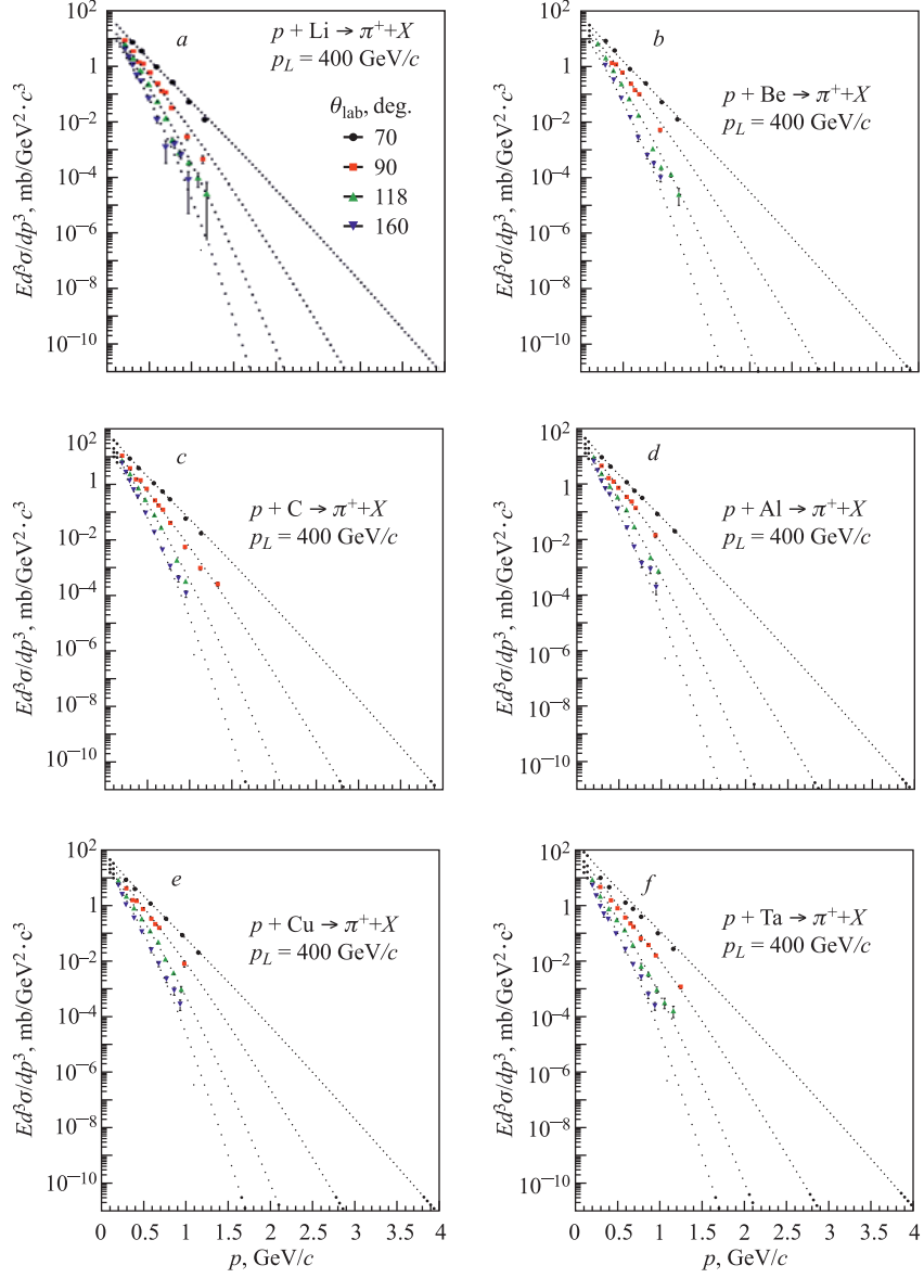
Fig. 4. Transverse momentum spectra of the \pi^+ mesons produced in p + A collisions at momentum p_L = 400 GeV/c and angle \theta_{\text{lab}} = 70, 90, 118 and 160^\circ in p presentation. The dotted lines are predictions based on z -scaling. The points are the experimental data taken from [27]
