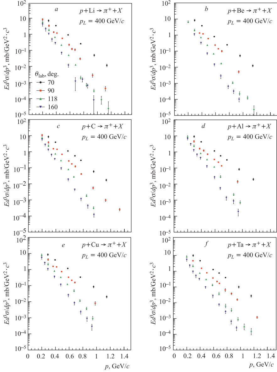
Fig. 1. Transverse momentum spectra of the \pi^+ mesons produced in p + A collisions at incident proton momentum p_L = 400 GeV/c and angle \theta_{\text{lab}} = 70, 90, 118 and 160^\circ in p presentation. The experimental data are taken from [27]
