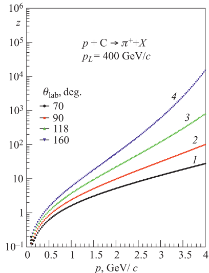
Fig. 6. z - p plot for p + C collisions at p_L = 400 GeV/ c . Dotted lines 1, 2, 3 and 4 correspond to \theta_{\text{lab}} = 70, 90, 118 and 160^\circ , respectively
